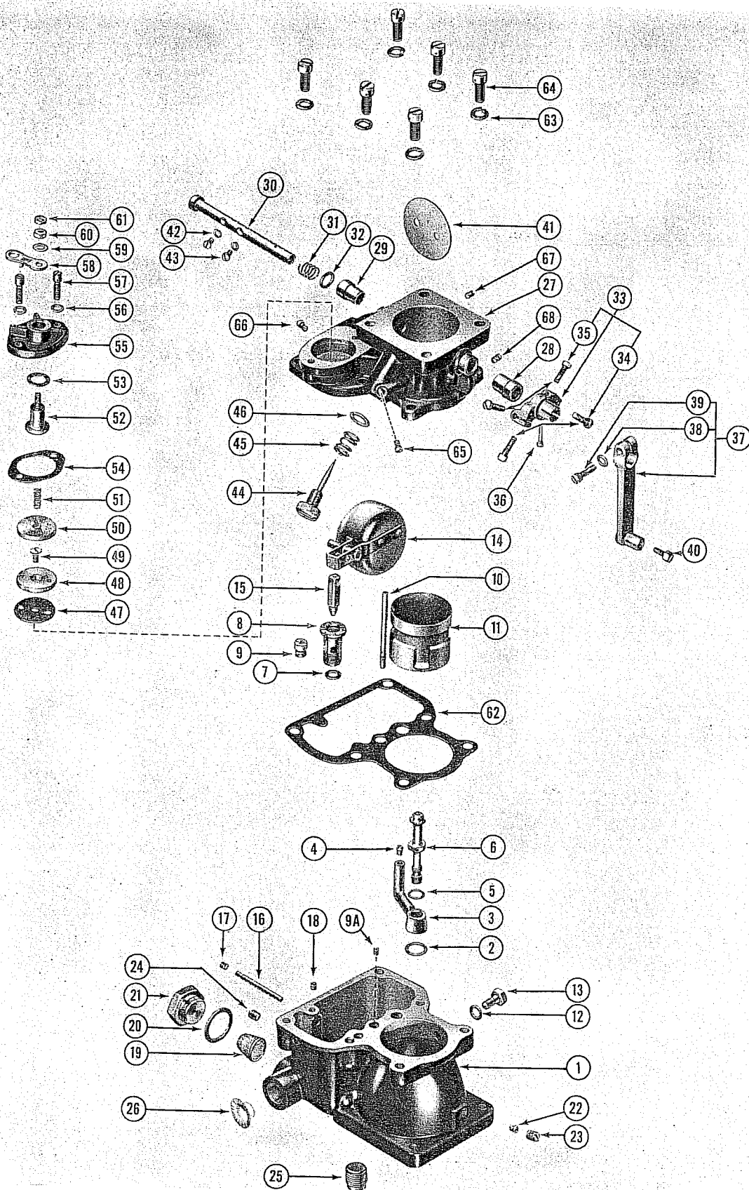
Figure 48 — Exploded View of Stromberg NA-S3A1 Series Carburetor
